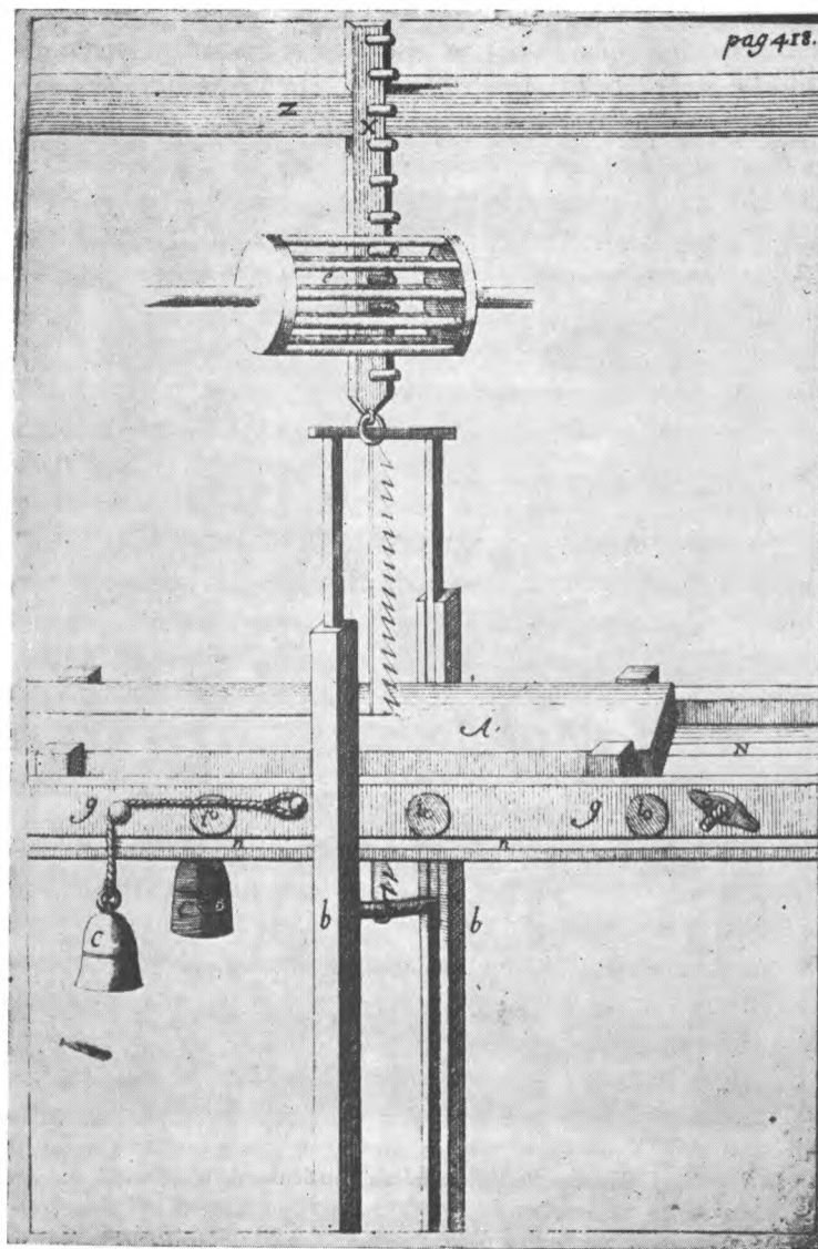
Engenho manual de serrar madeira (c. 1730)
